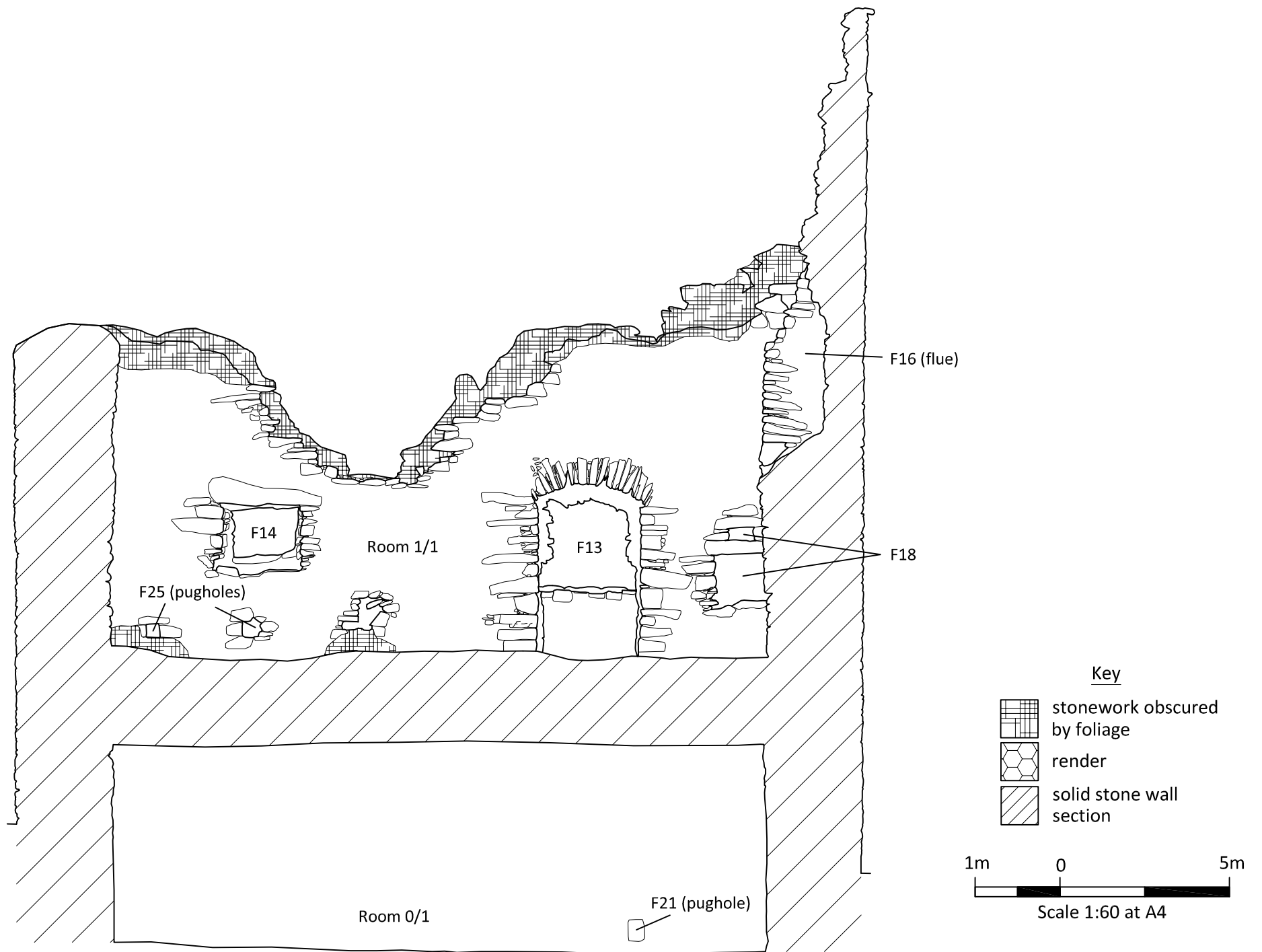
Figure 20: Rooms 1 / 1 and 0 / 1, north-east elevation
