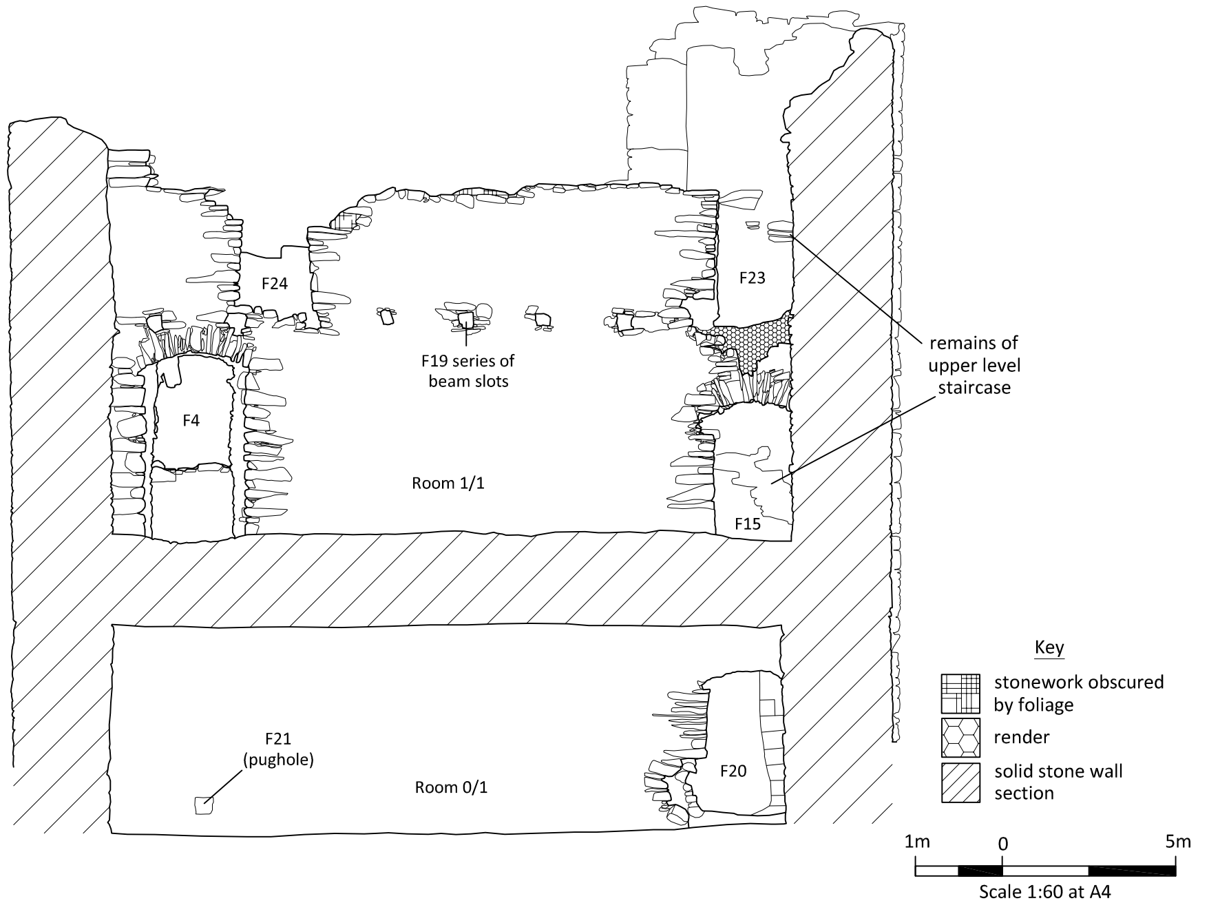
Figure 18: Rooms 0/1 and 1/1, south-west elevations
